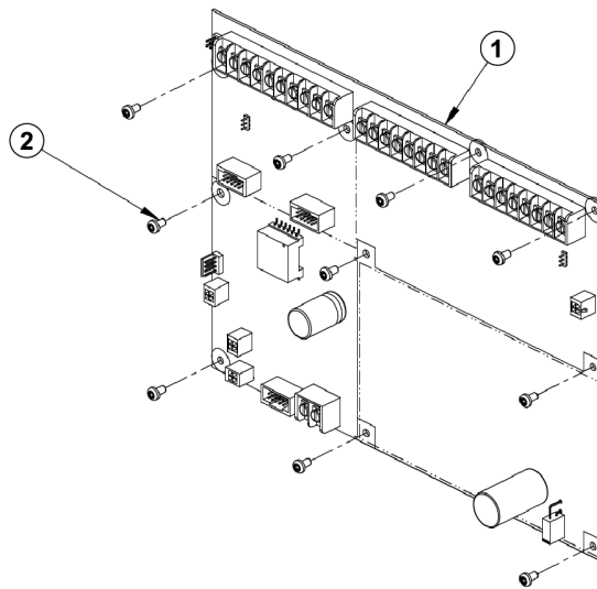
Figure 3: 650-1244 NAC Power Supply board
