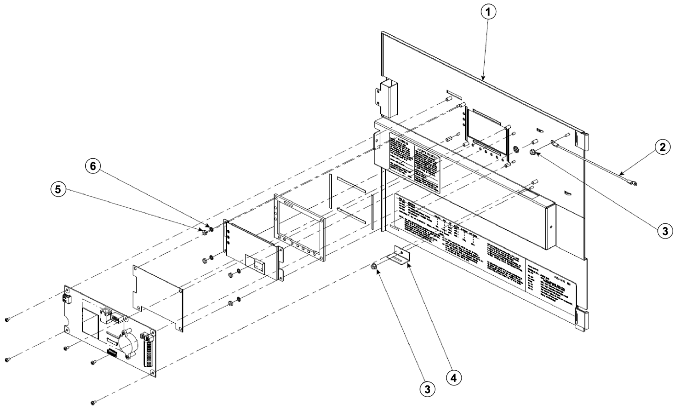
Figure 1: Front assembly with electronics
