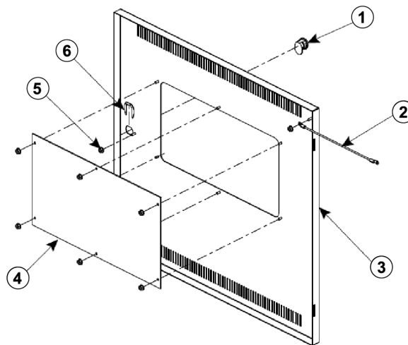
Figure 4: Door assembly
