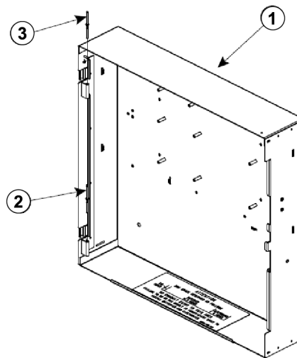
Figure 2: 699-549 Backbox assembly
